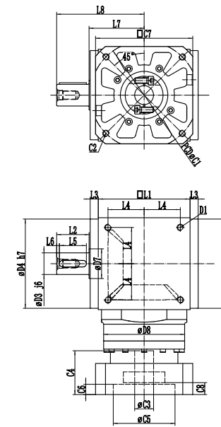
Dimension (double stage, Ratio i=4\sim 20 )
